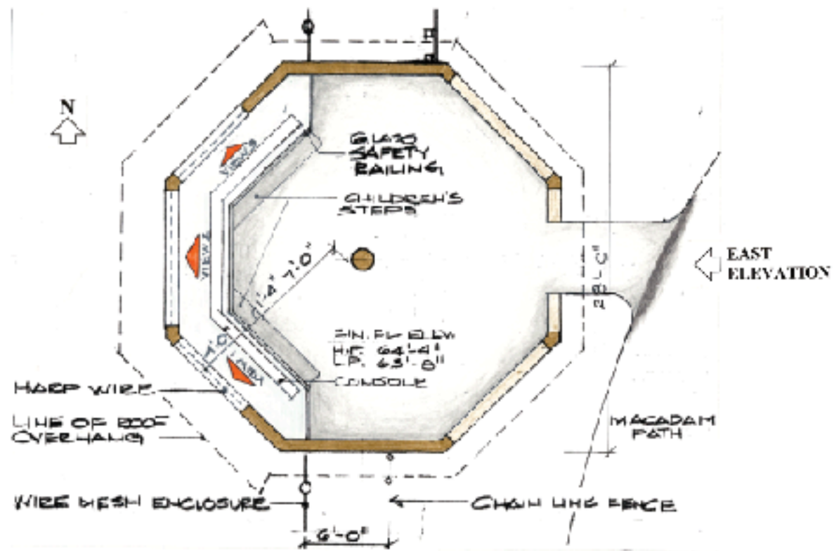
Pavilion Number 1 - Plan
