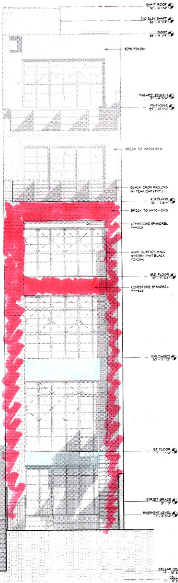
NORTH ELEVATION - PROPOSED
