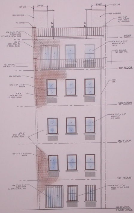
PROPOSED @ REAR ELEVATION SCALE 1/4"=1'-0"
