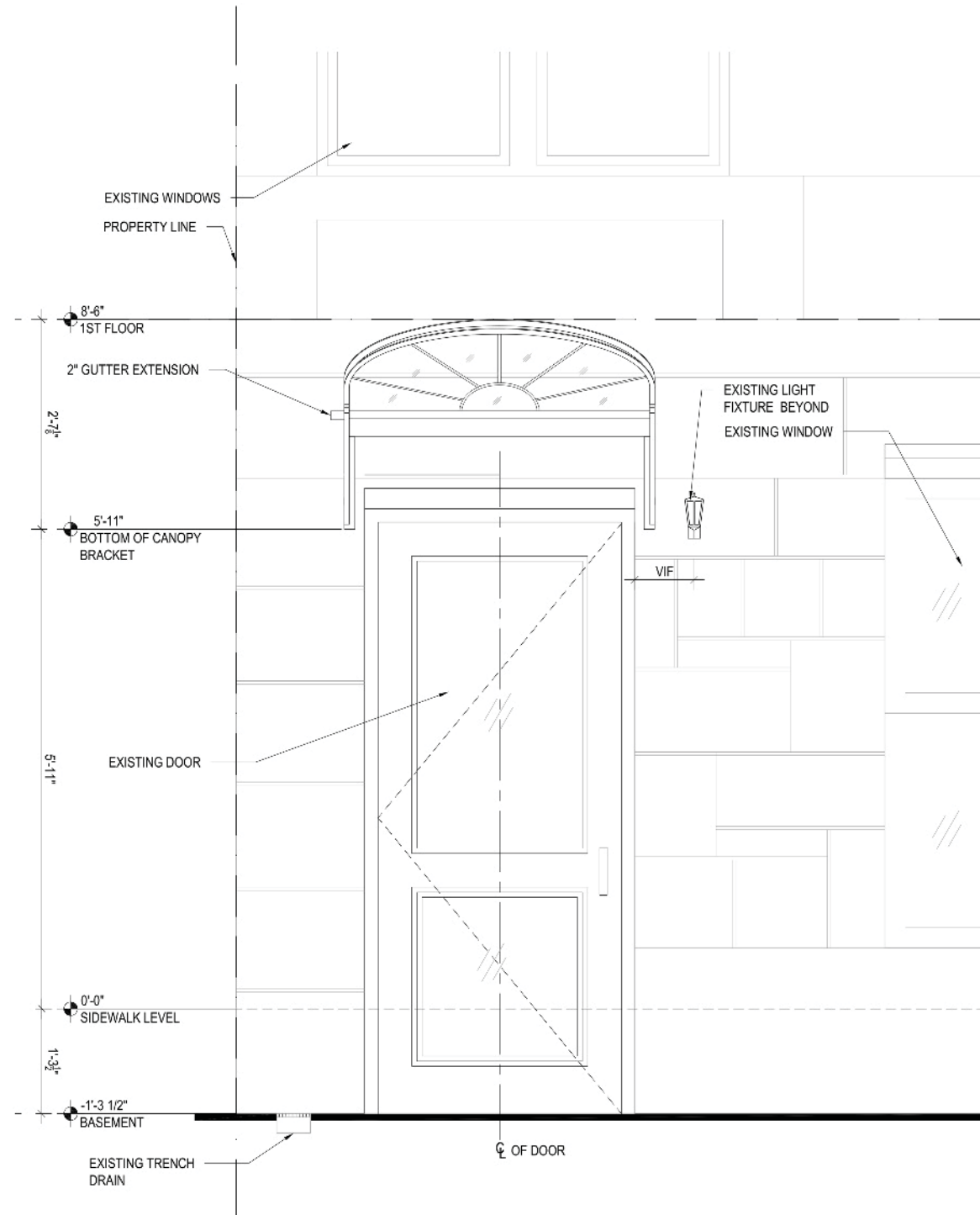
Elevation of Proposed Canopy- 36 W 94 th St
