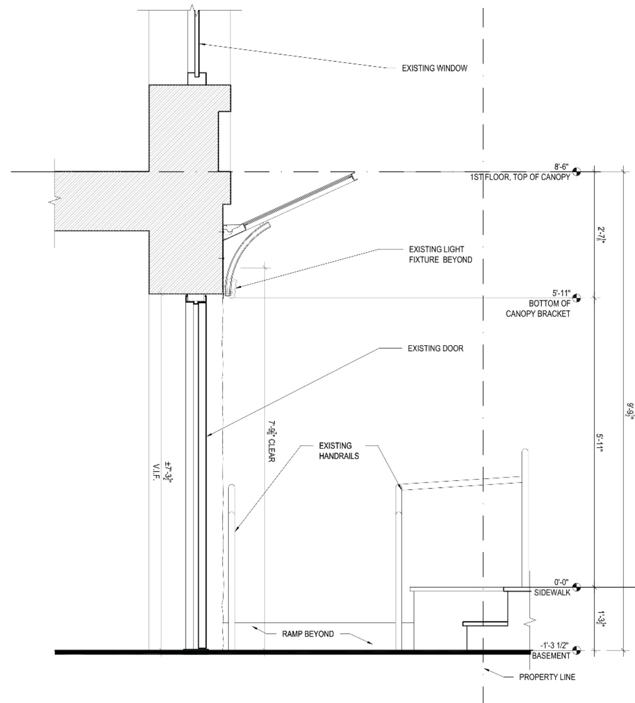
Section of Proposed Canopy- 36 W 94 th St
