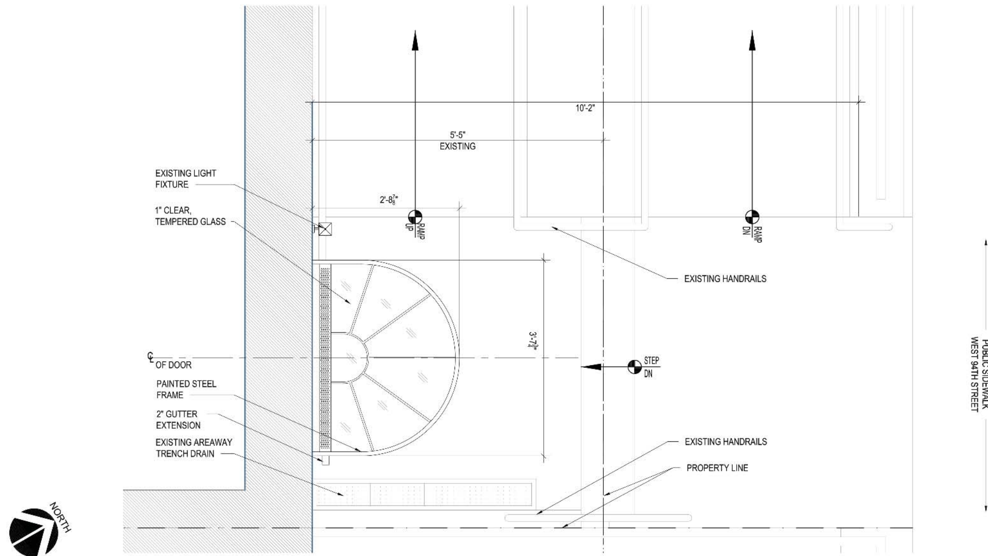
Plan of Proposed Canopy- 36 W 94 th St
