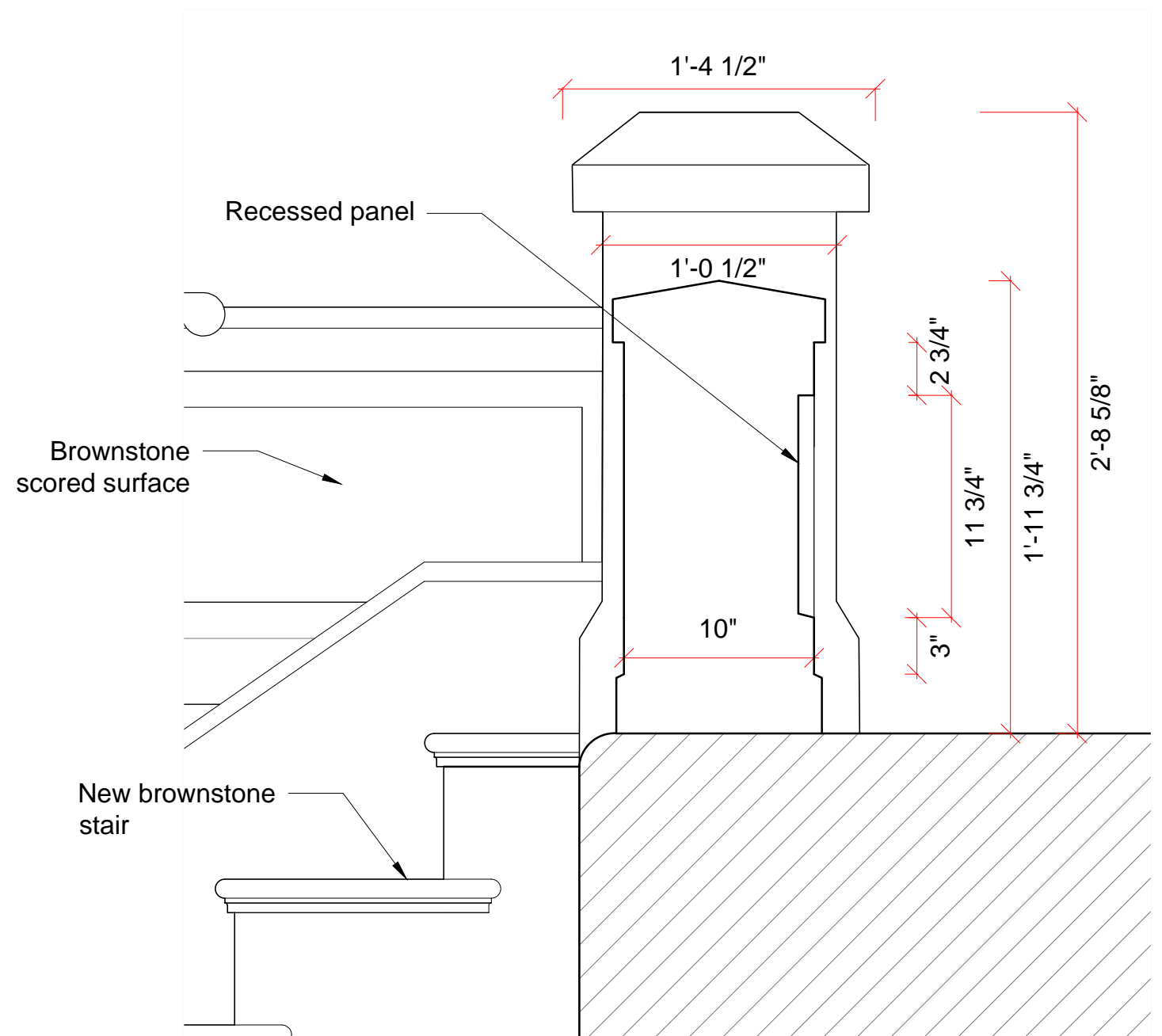
Areaway section
