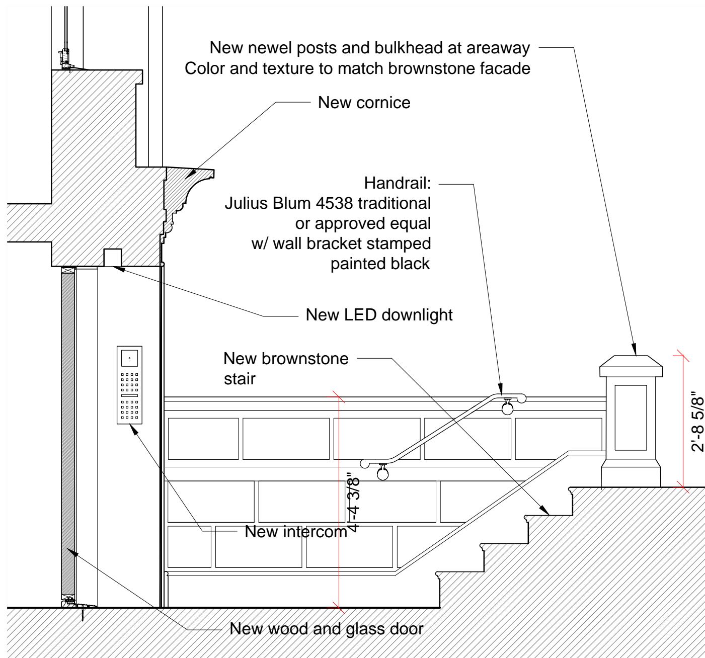
Areaway section
