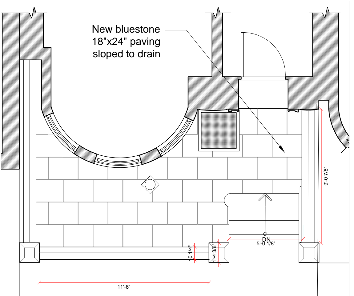
Areaway floor plan
