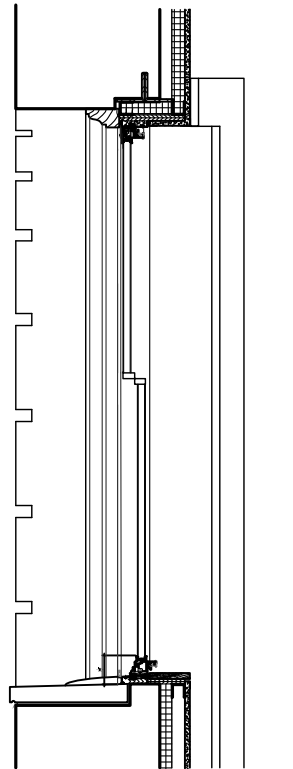
2 SECTION @ STRAIGHT WALL 1/2" = 1'-0"
