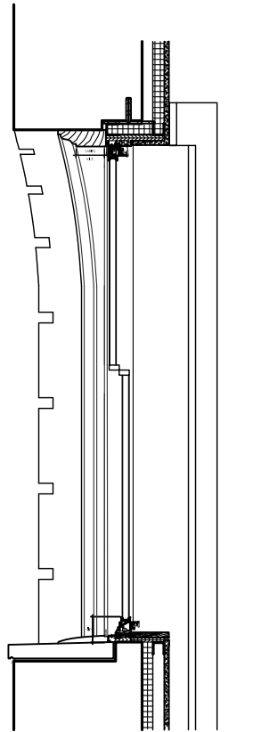
2 SECTION @ CURVED WALL 1/2" = 1'-0"
