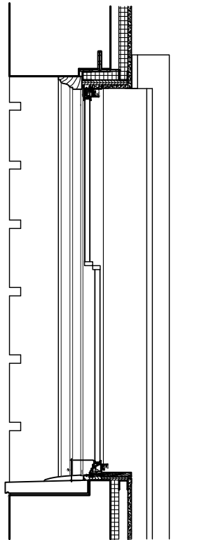
2 SECTION @ STRAIGHT WALL 1" = 1'-0"
