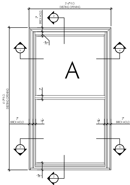
1 LANDMARK WINDOW ELEVATION A 1/2" = 1'-0"
