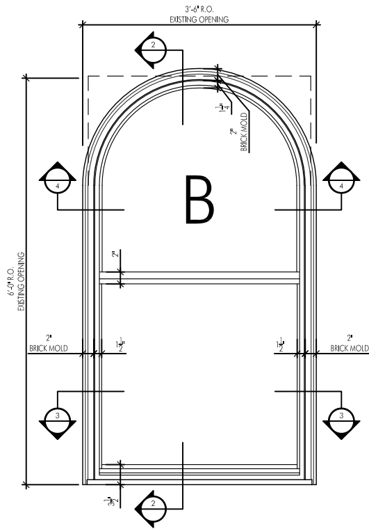
1 LANDMARK WINDOW ELEVATION B 1/2" = 1'-0"
