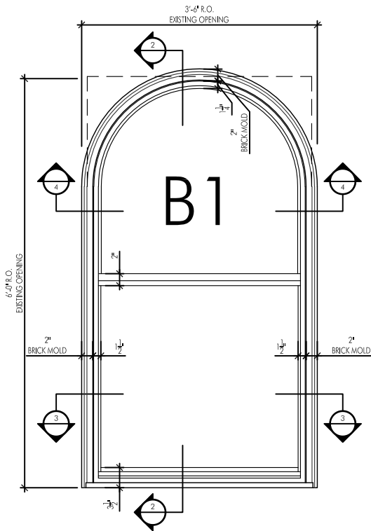
1 ELEVATION 1/2" = 1'-0"
