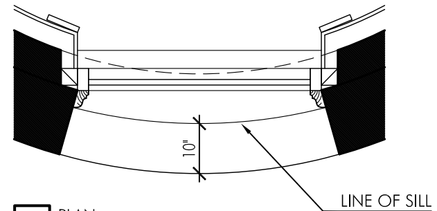
3 PLAN 1/2" = 1'-0"
