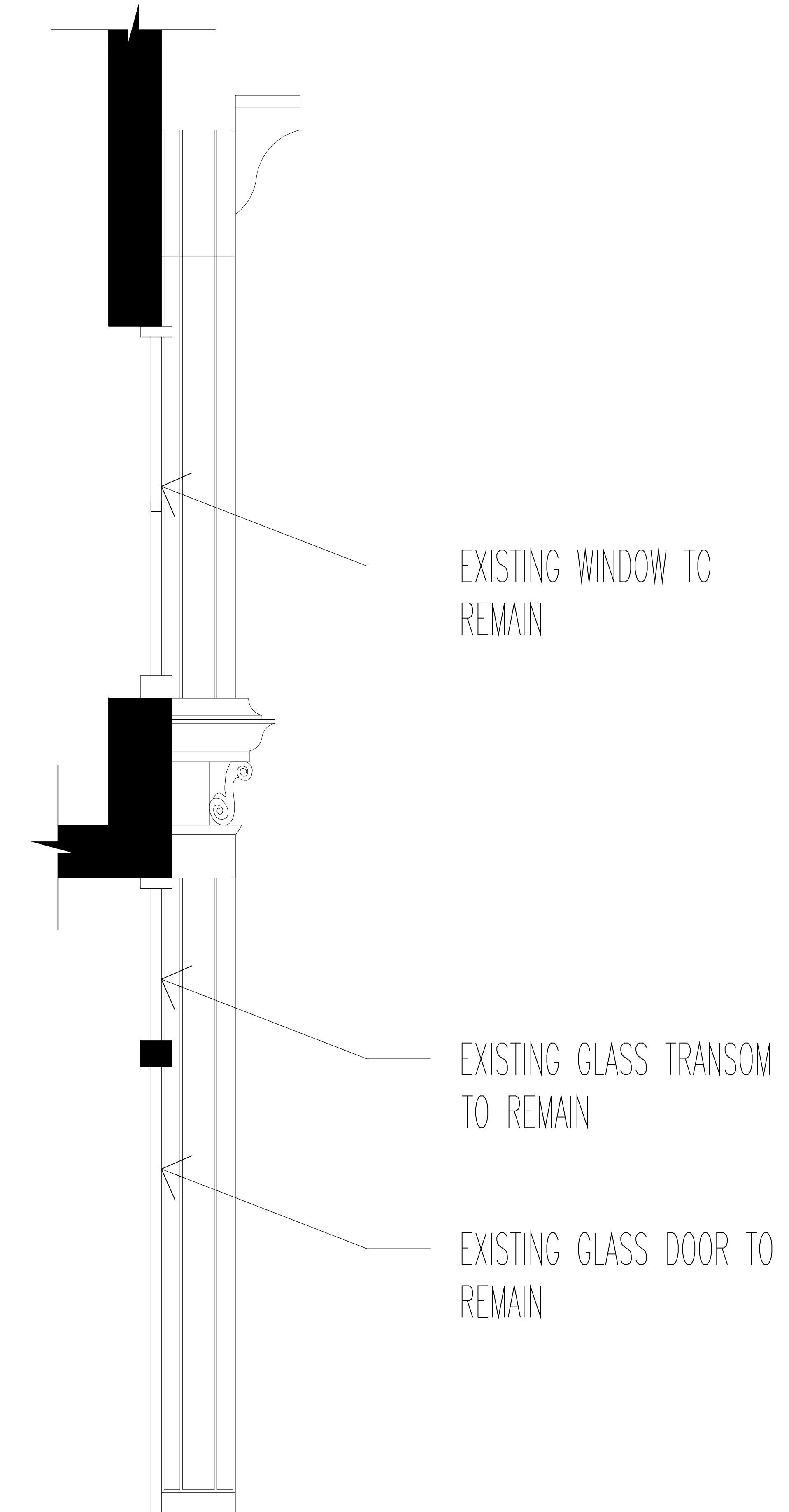
EXISTING ENTRY SECTION
