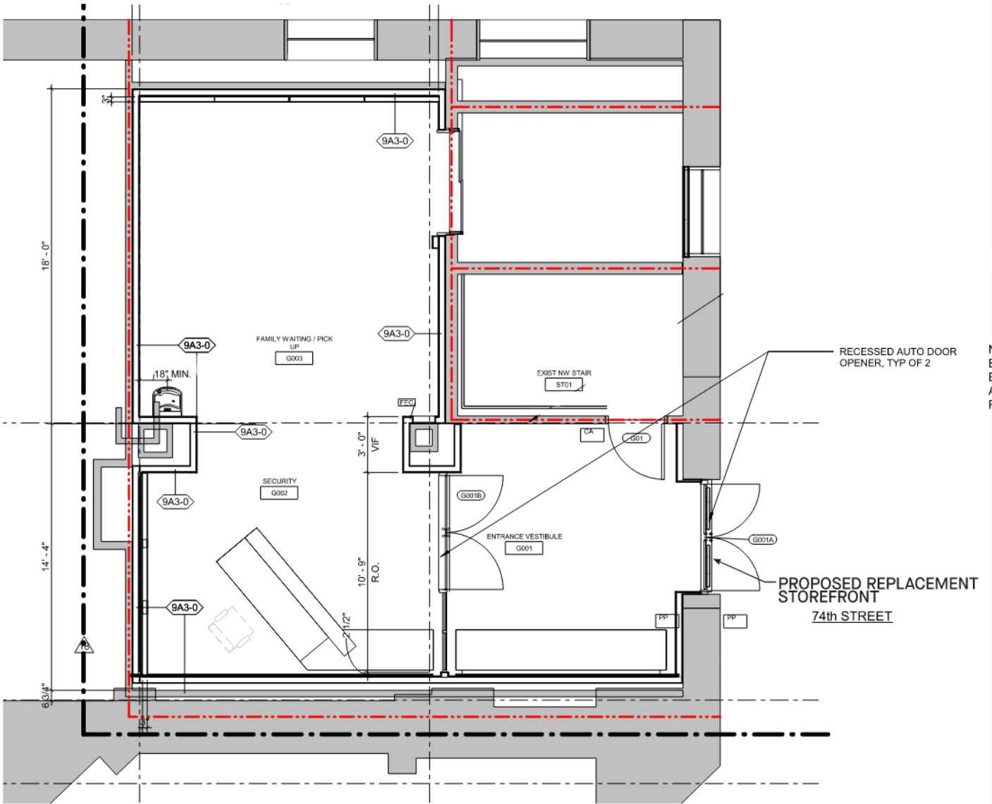
8 PROPOSED GROUND PLAN
