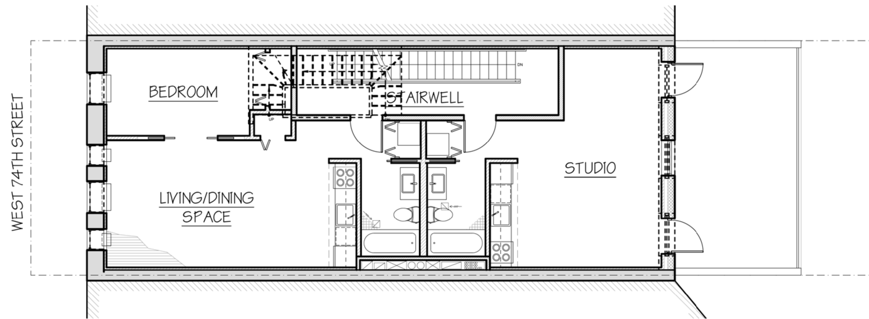
APPROVED 4TH FLOOR PLAN
