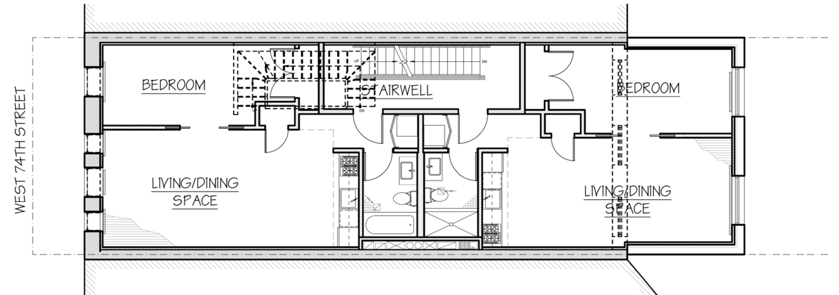
PROPOSED 4TH FLOOR PLAN
