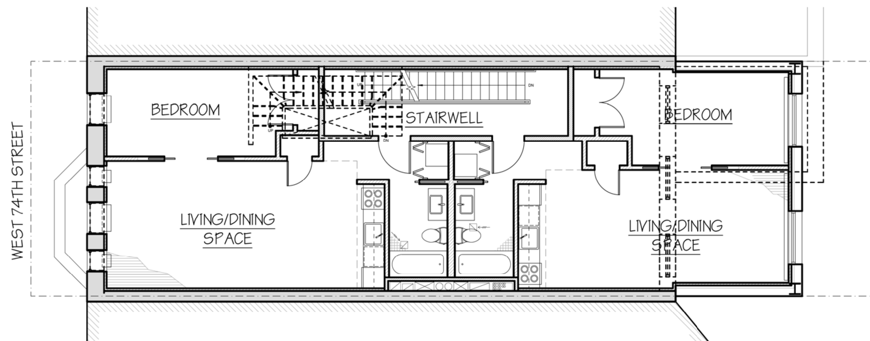
APPROVED 2ND/3RD FLOOR PLAN
