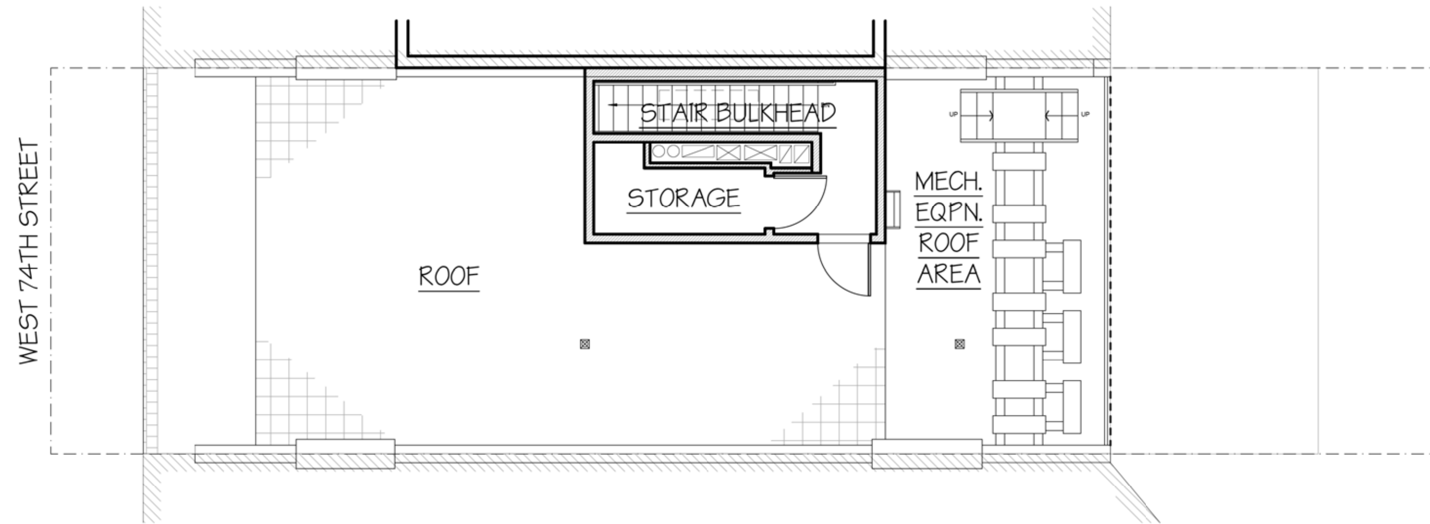
APPROVED ROOF PLAN
