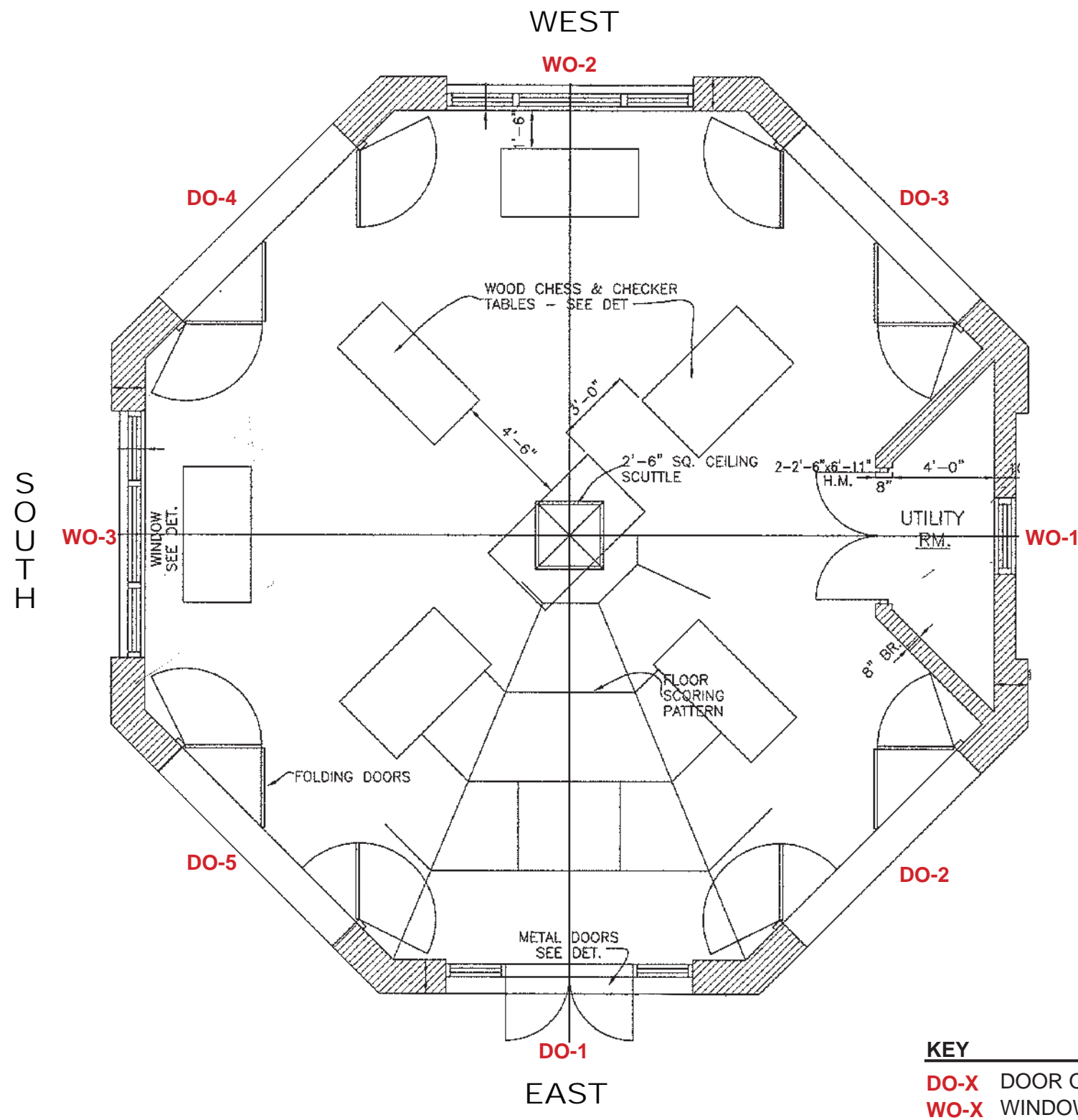
1952 FLOOR PLAN
