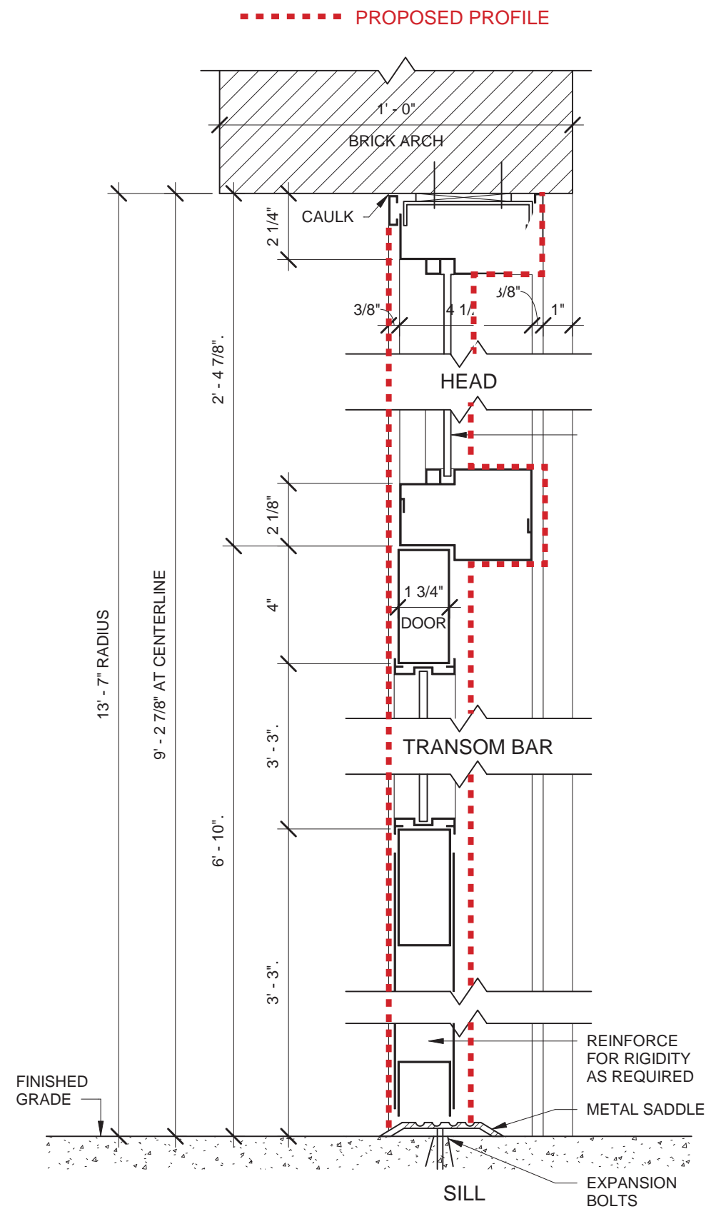
EXISTING DOOR SECTION A-A WITH PROPOSED OVERLAY
