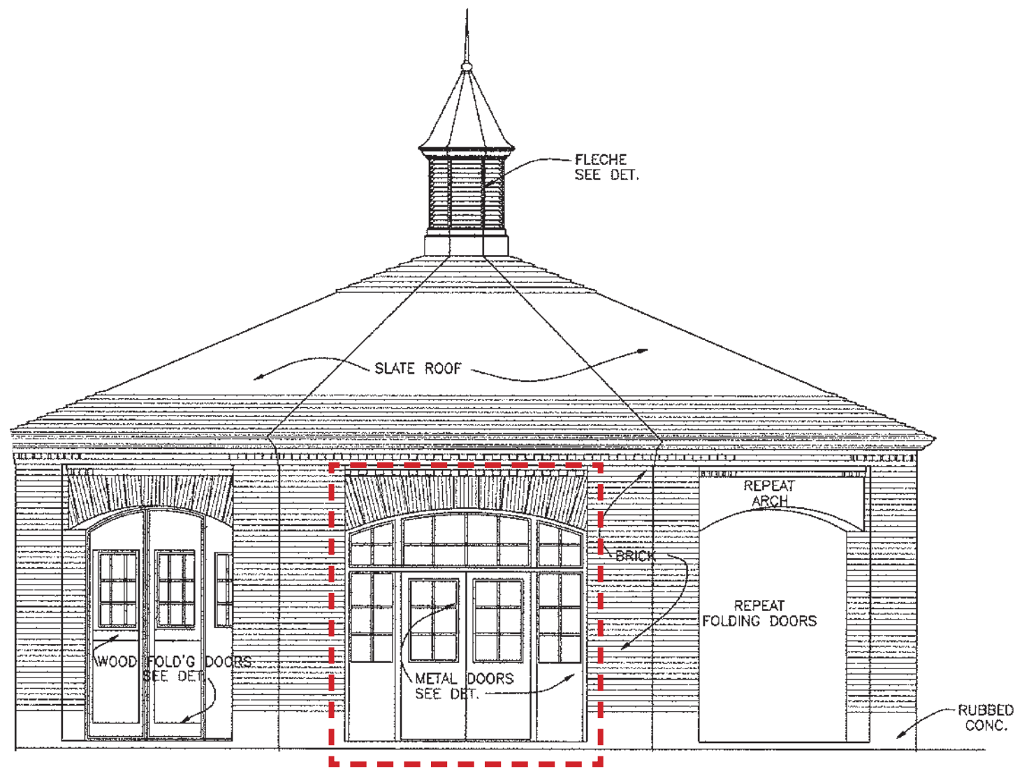
1952 ELEVATION
