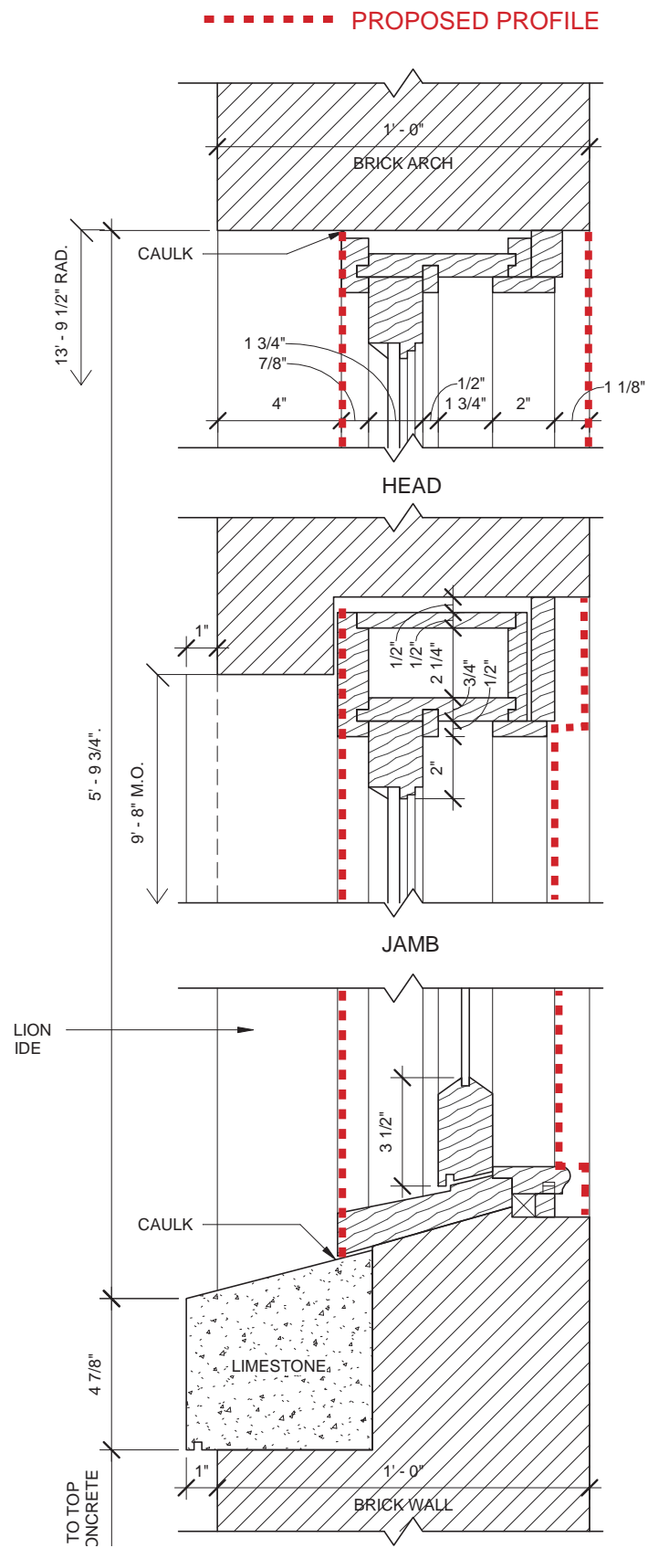
EXISTING WINDOW SECTION B-B WITH PROPOSED OVERLAY
