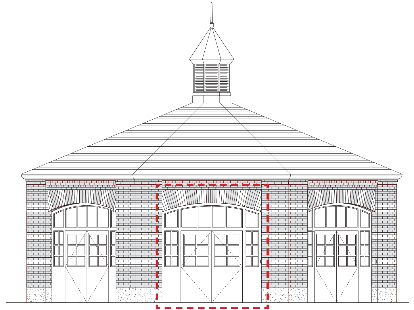
EXISTING ELEVATION
