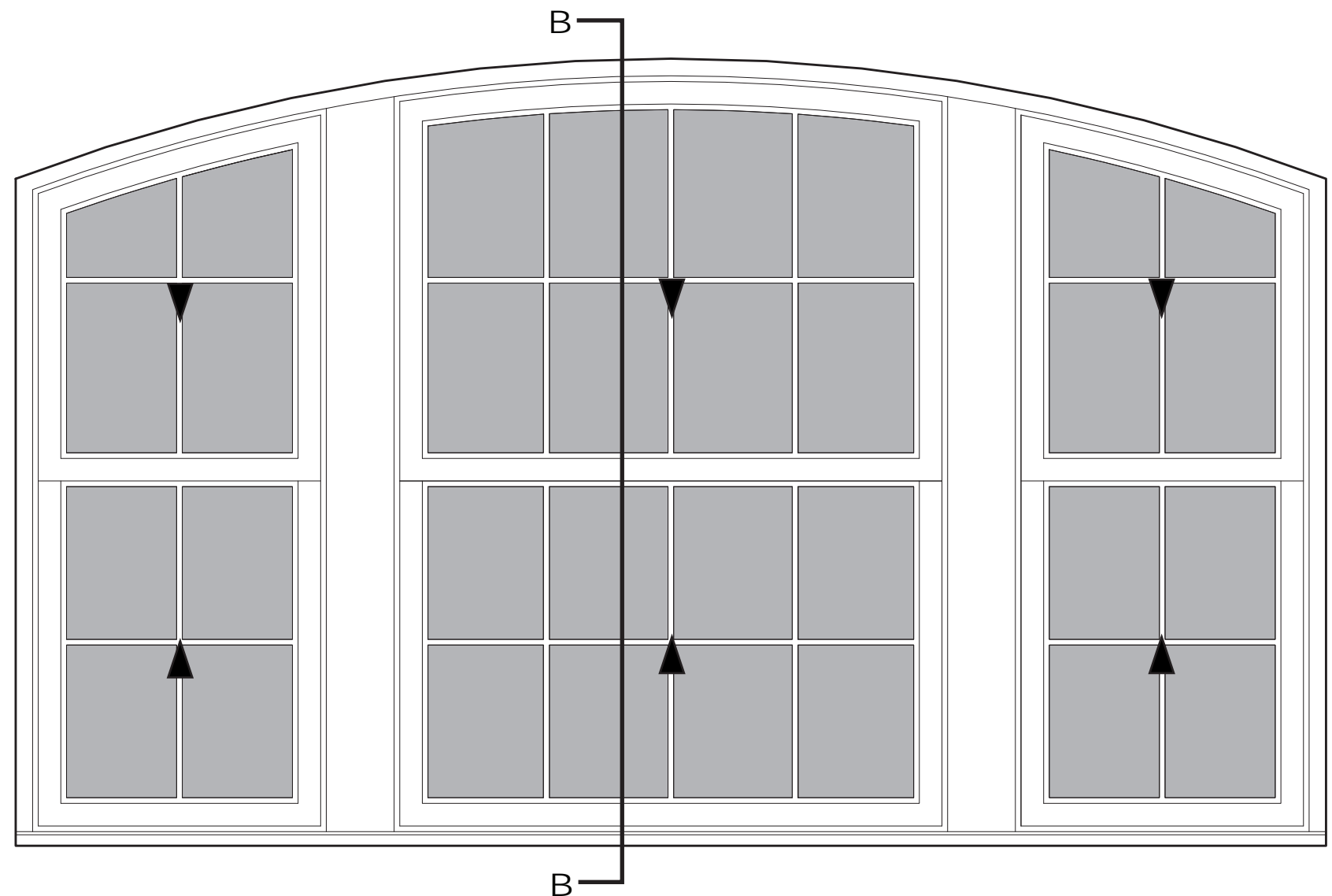
PROPOSED DOUBLE HUNG WINDOW ELEVATION (TO MATCH EXISTING)
