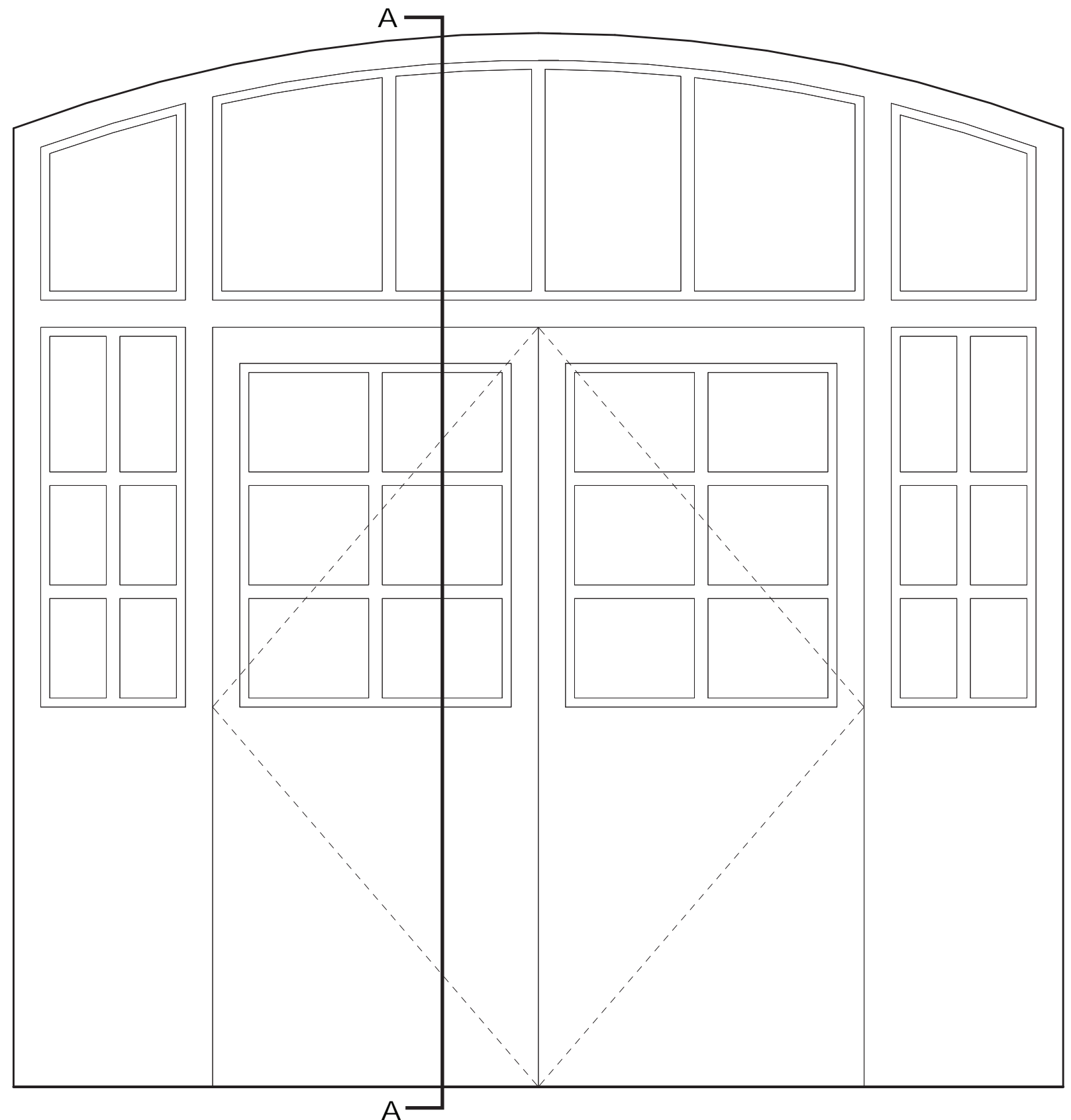
PROPOSED DOOR ELEVATION (TO MATCH EXISTING)
