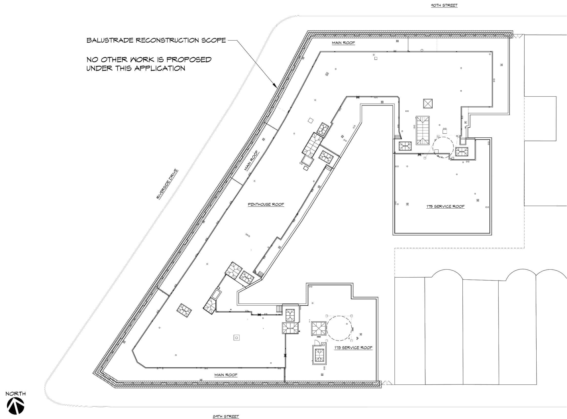
Roof plan indicating the scope of balustrade reconstruction (100% of street frontage)
