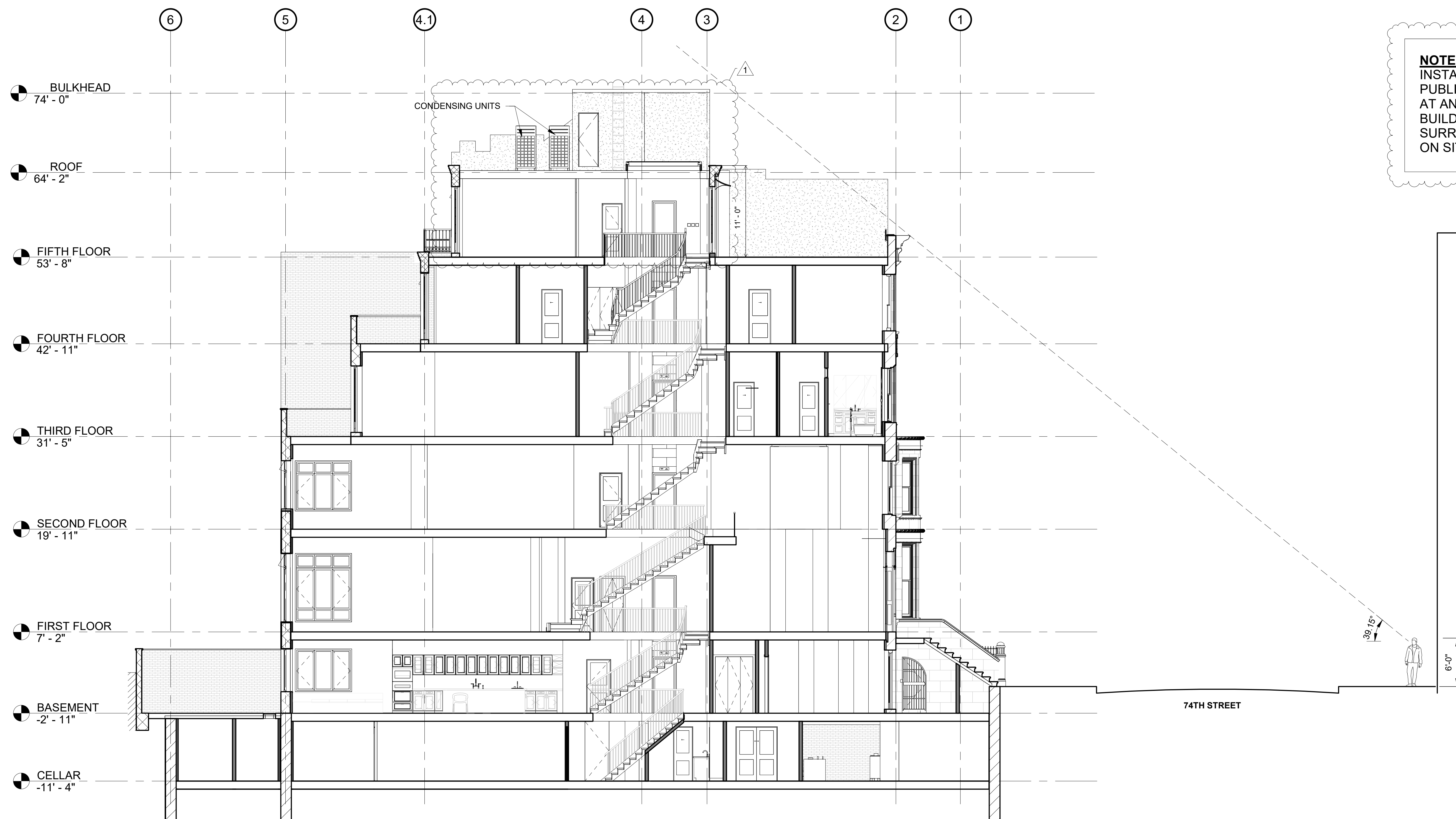
1 | SIGHTLINE SECTION NTS
