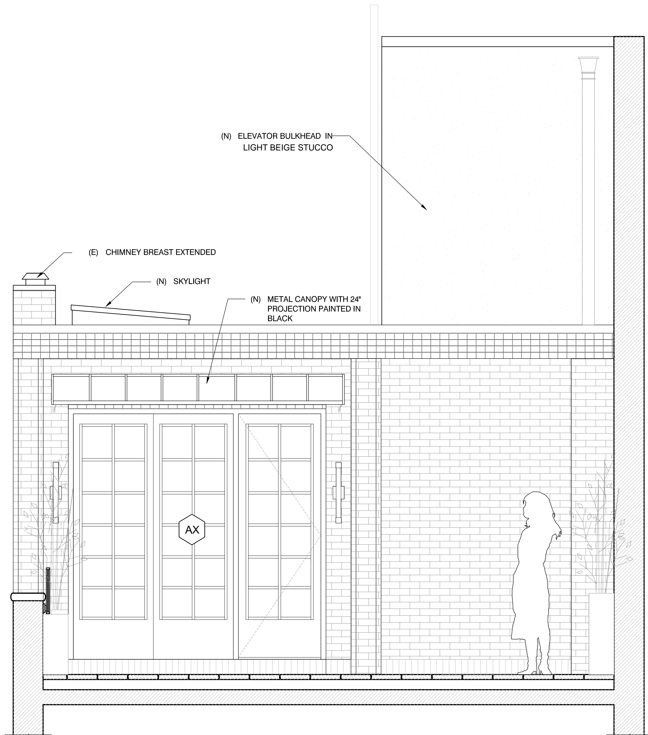
1 | FIFTH FLOOR FRONT ELEVATION NTS
