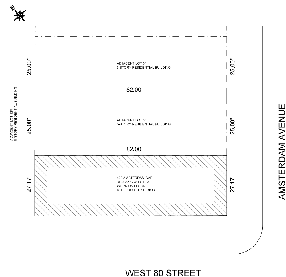
PLOT PLAN
